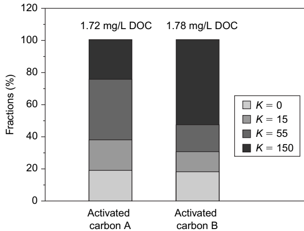
Figure 4.30 Application of the adsorption analysis for comparison of adsorbents ( K in [\text{mg C/g}]/[\text{mg C/L}]^n ).
